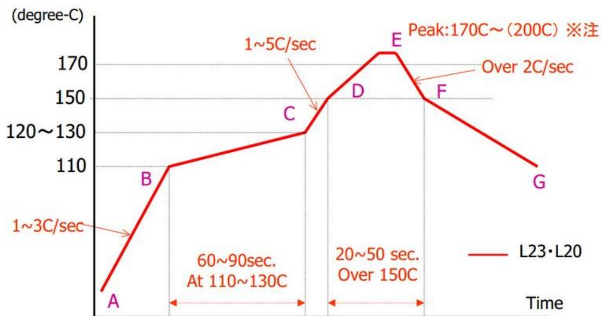
Figure 6.3 MAX2001 Module Solder Profile
