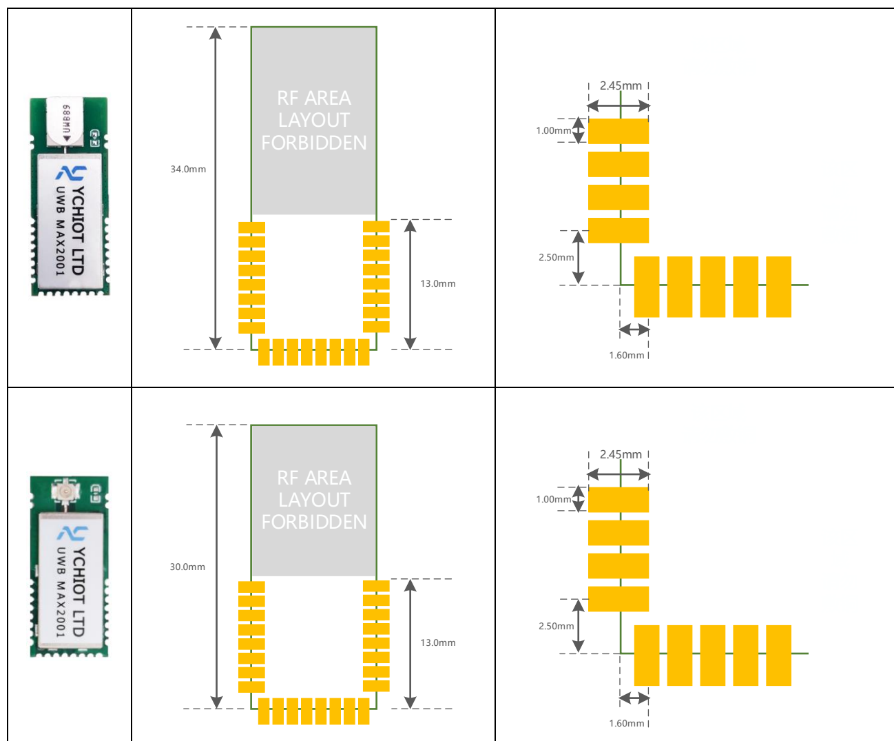
Figure 6.2 MAX2001 Module Land Pattern (Unit: mm)
