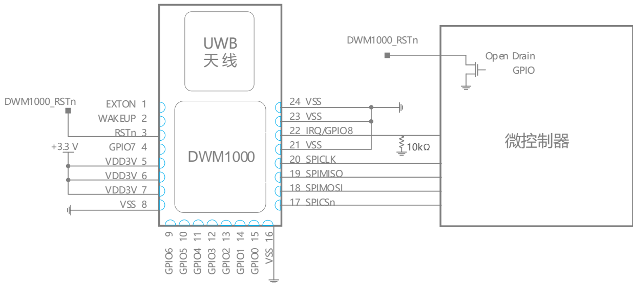
Figure 9: Example DWM1000 Application Circuit
