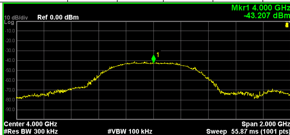
DWM1000-SMA Channel 2
