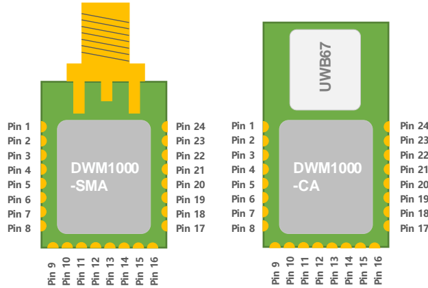
Figure 5: DWM1000 Pin Diagram
