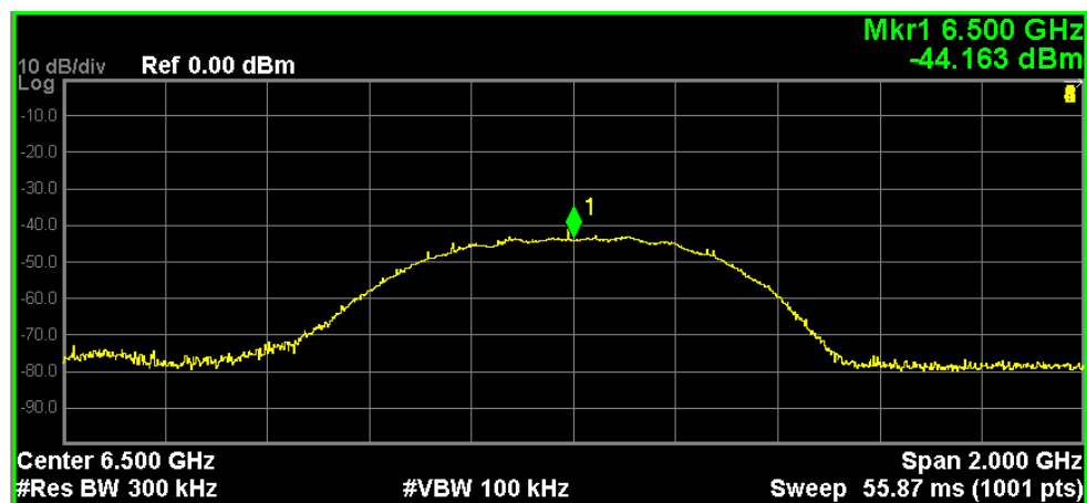
DWM1000-SMA Channel 5
