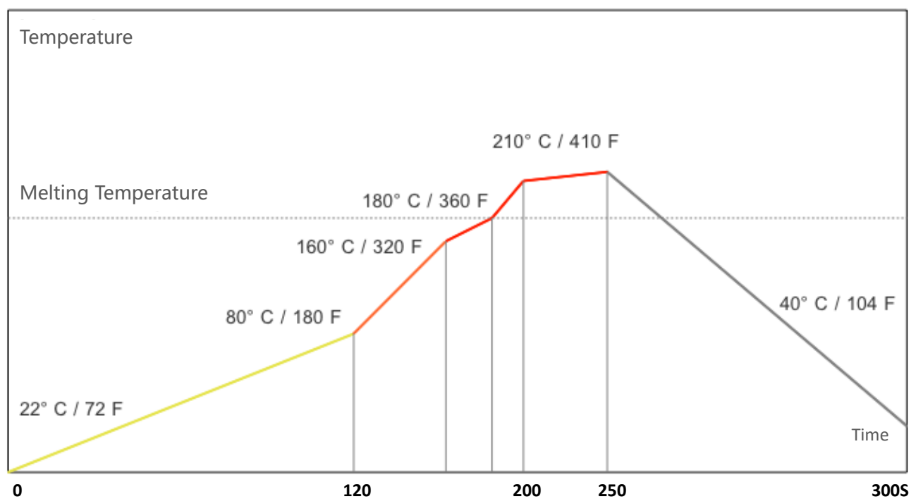
Fig 6.3 Reflow temperature curve of DWM1000 module
