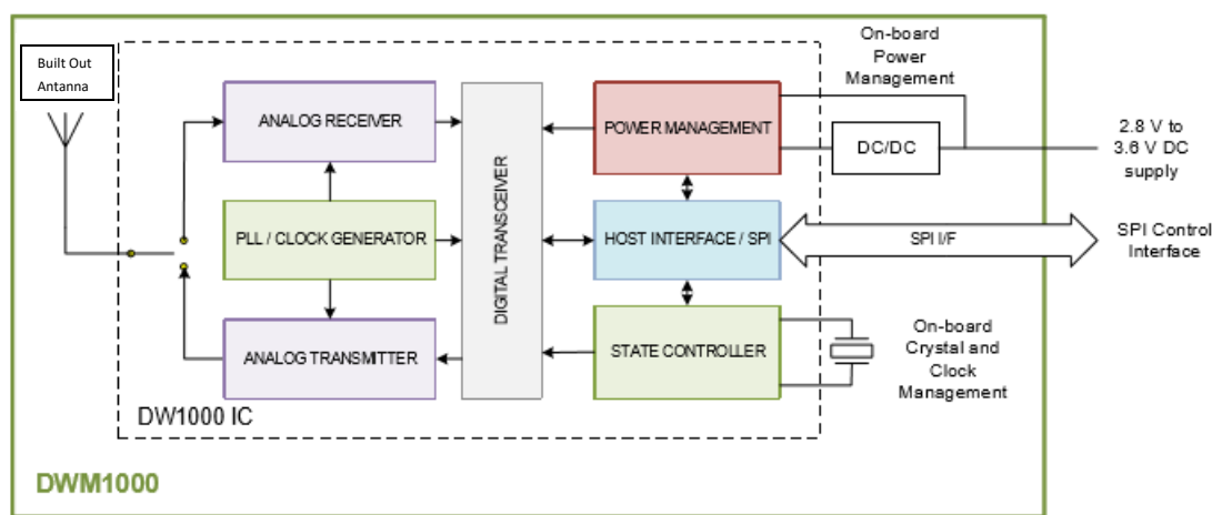
High Level Block Diagram
