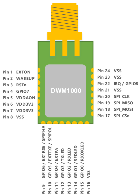
Figure 5: DWM1000 Pin Diagram
